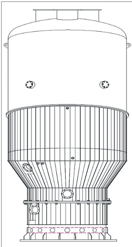
Fig. 7: Construction drawing of the shaft furnace where cooling of the lower part of the shaft is realized with ILTEC Technology
