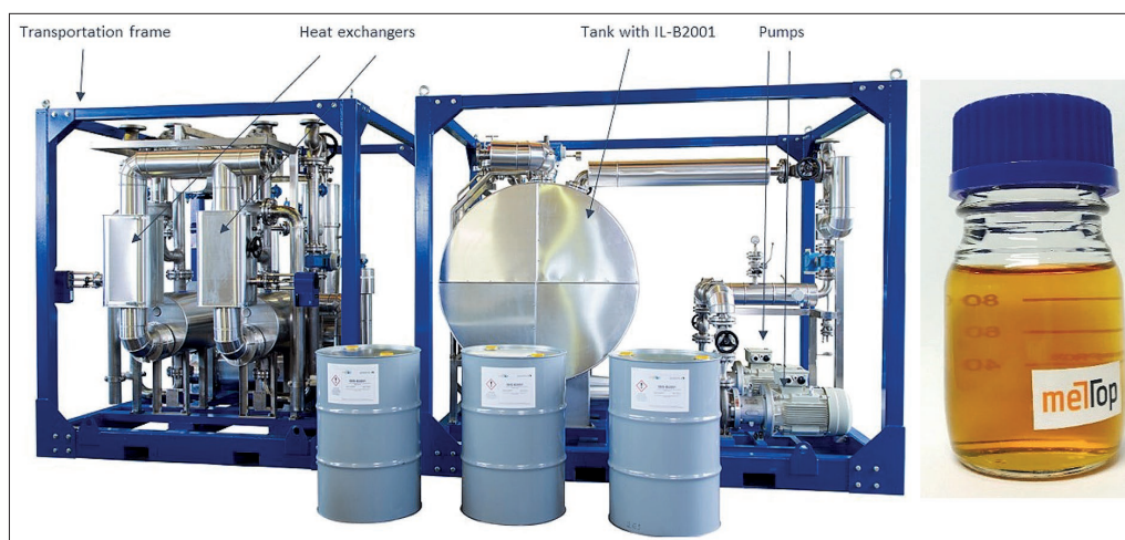
Fig. 4: Basic design of an ILTEC system as installed at ArcelorMittal Bremen GmbH in Germany (left) and photo of the optical appearance of the ionic liquid IL-B2001
