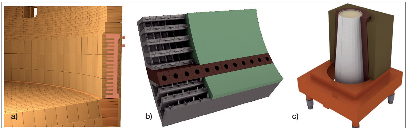
Fig. 8: Three examples of a breakthrough way to increase furnace availability by cooling beneath bath level: High intensity cooler within the lining of side wall of an electric arc furnace (a), cooling concept of tuyere zone in a Peirce Smith Converter (b) and cooling of a purging plugs in an anode furnace (c)
