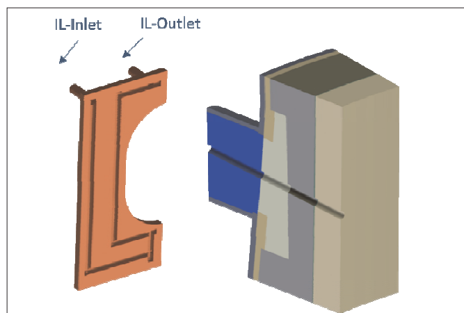
Fig. 6: Special design of the cooled tap hole with the copper cooled back plate mounted upon the steel shell
