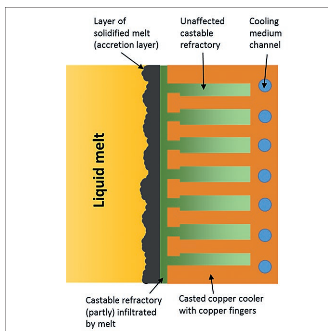
Fig. 1: Schematic picture of the entire cooling system (high intensity cooling with a freeze lining concept)
