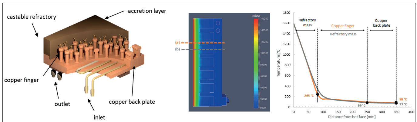
Fig. 3: Special design of a composite furnace module cooling (CFM) element for creating a freeze lining (left) and CFD modelling of the temperature distribution at a furnace temperature of 1600 °C (middle) and resulting steep temperature gradient within the refractory mass (right)
