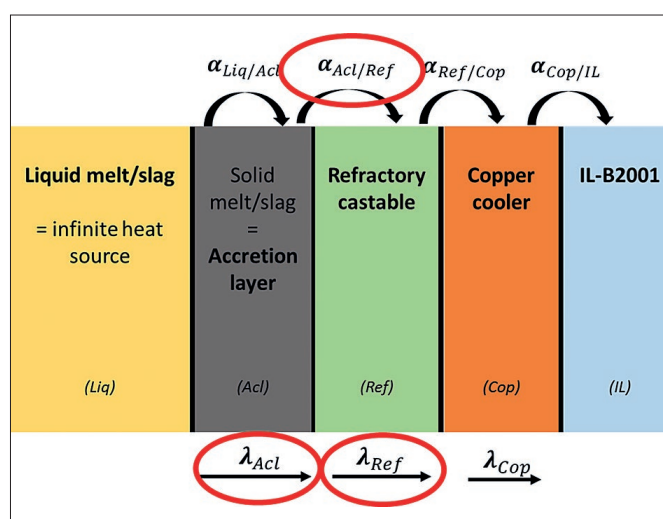
Fig. 2: Limiting factors for heat transfer for the system as given in Figure 1
